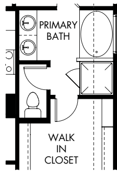
② OPT. SHOWER/TUB COMBO
