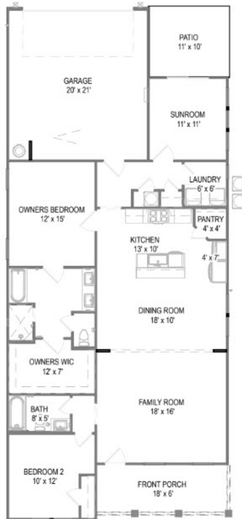
First Floor
