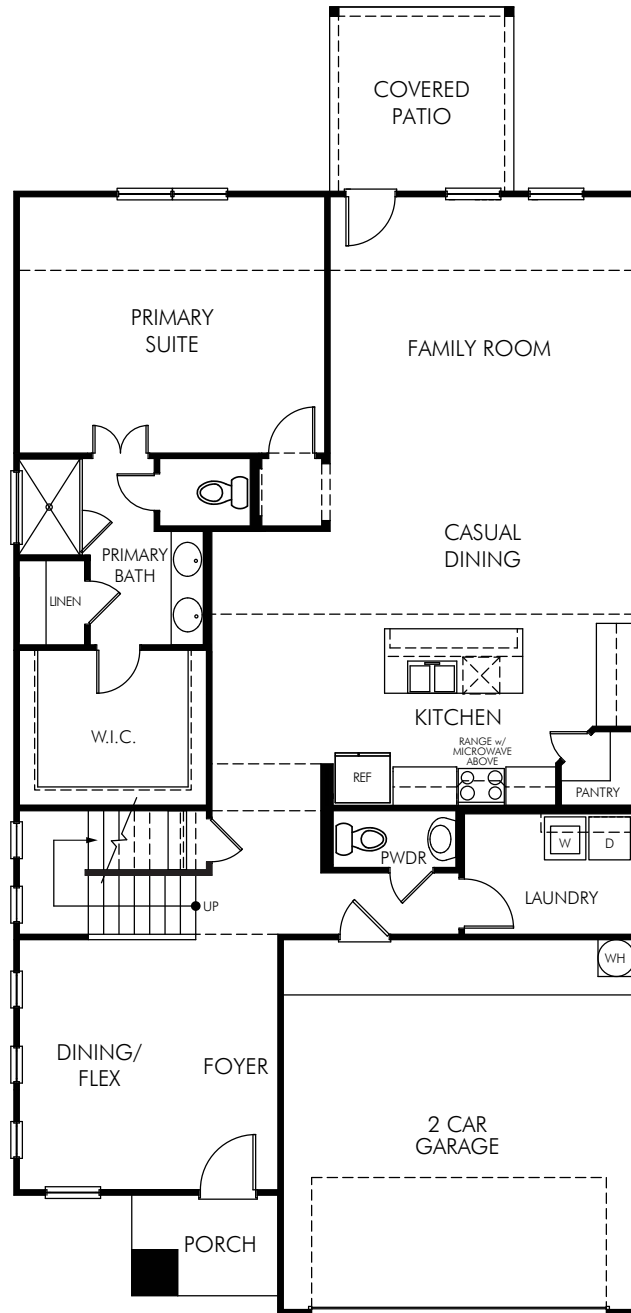
The Texoma | Plan 3L08 | First Floor Approx. 2,738 sq. ft. | 4 Bed | 3.5 Bath | 2 Car Garage | 2 Story
