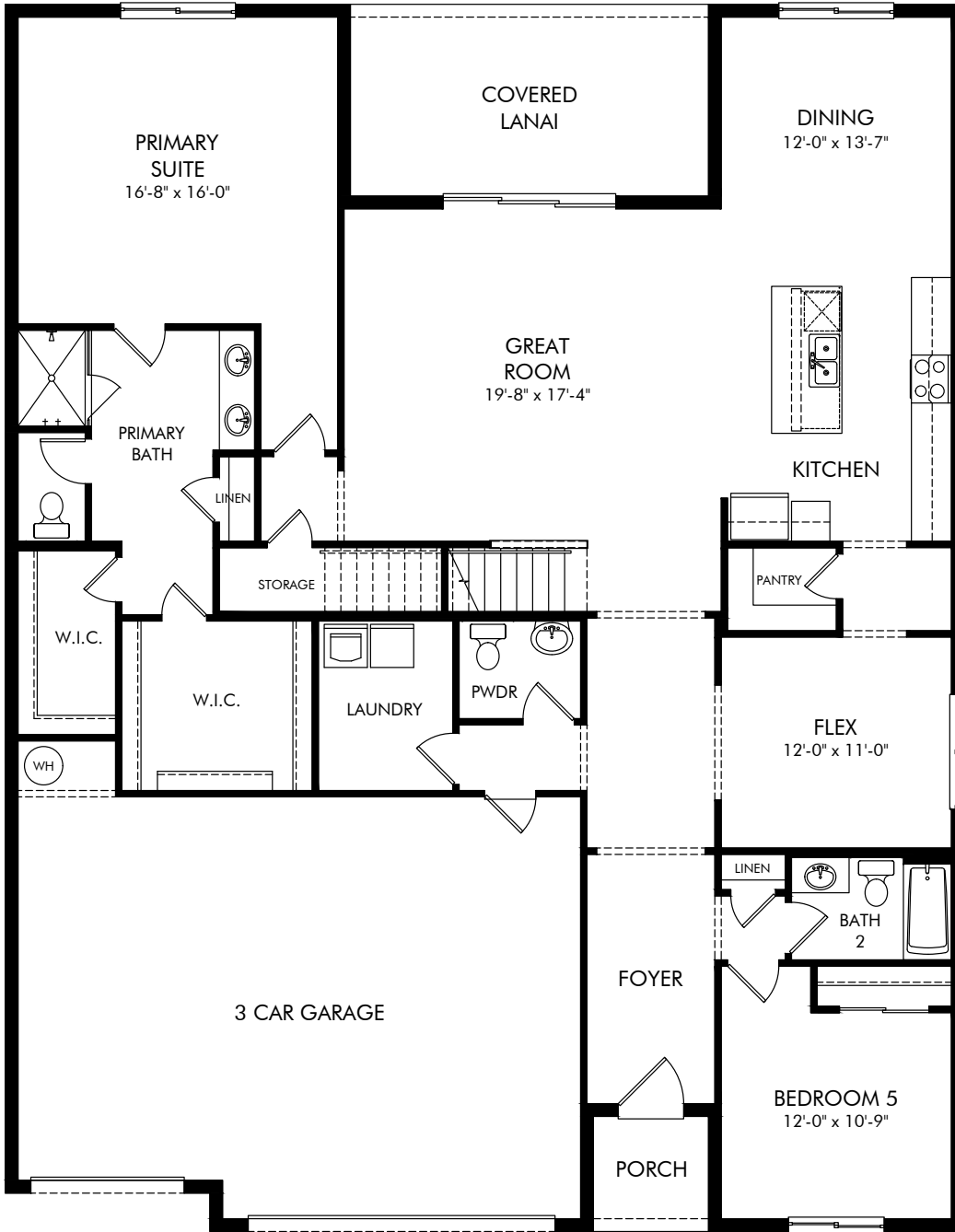
Two Rivers - Signature Series | Zander | First Floor Approx. 3,807 sq. ft. | 5 Bed | 4.5 Bath | 3 Car Garage | 2 Story
