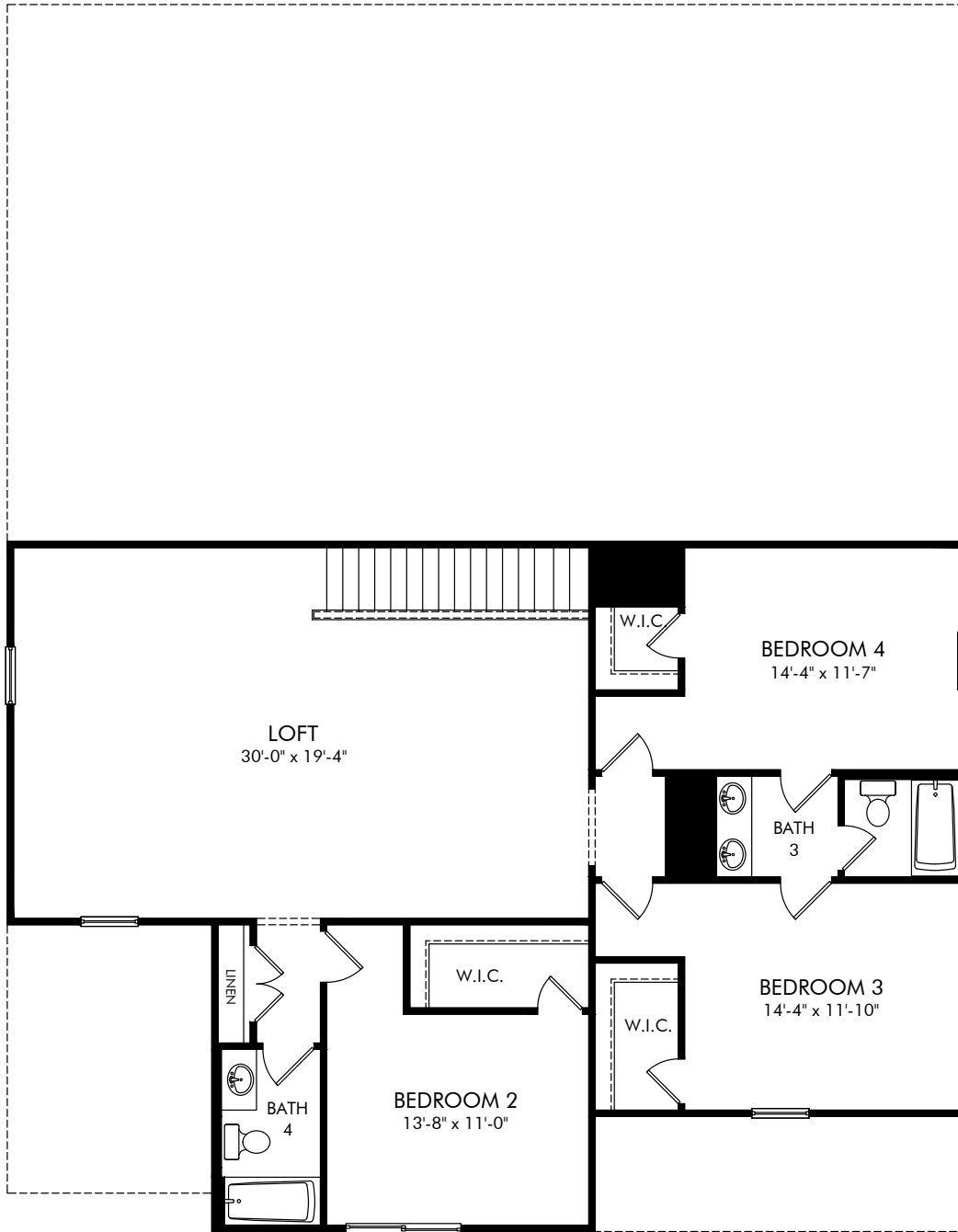
Two Rivers - Signature Series | Zander | Second Floor Approx. 3,807 sq. ft. | 5 Bed | 4.5 Bath | 3 Car Garage | 2 Story
