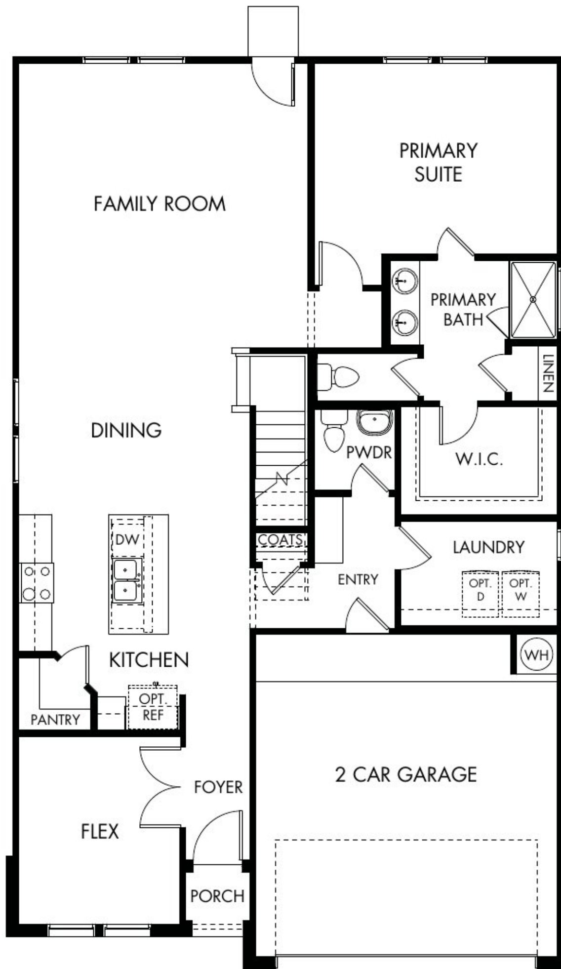
Thomas Pond | The Matador | Plan 870 | First Floor Approx. 2,404 sq. ft. | 4 Bed | 2.5 Bath | 2 Car Garage | 2 Story
