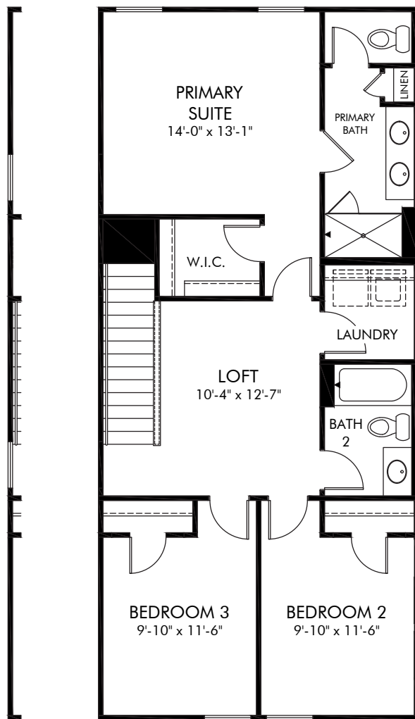
END UNIT
